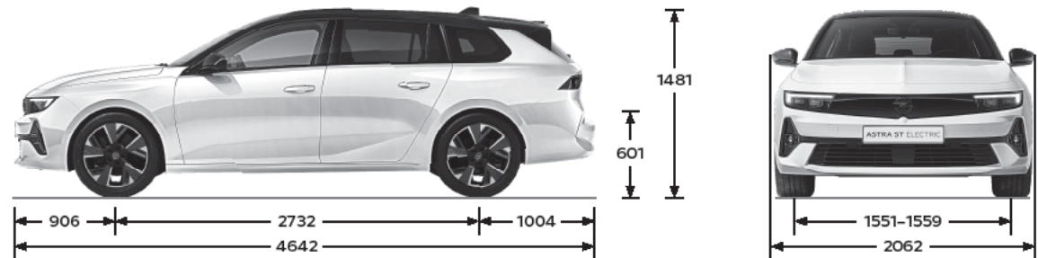
All dimensions in mm
